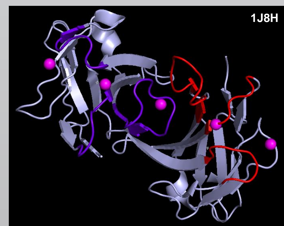
V(D)J region of the TCR of structure 1J8H. View from the CDRs towards the constant region (Above). View from the side of the TCR (below). Pink spheres = Linear regression vector of the CDRs of structure 1J8H. Purple = CDRa's. Red = CDRb's. Teal = TCR V(D)J center of mass
